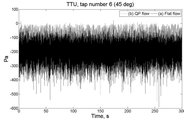
Fig. 7 Typical roof pressure time history data under (a) flat wind flow and (b) quasi-periodic (QP) wind flow
