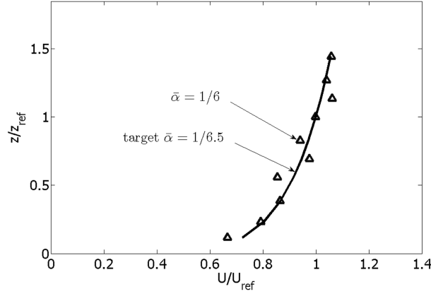
Fig. 4 Mean wind speed profile
