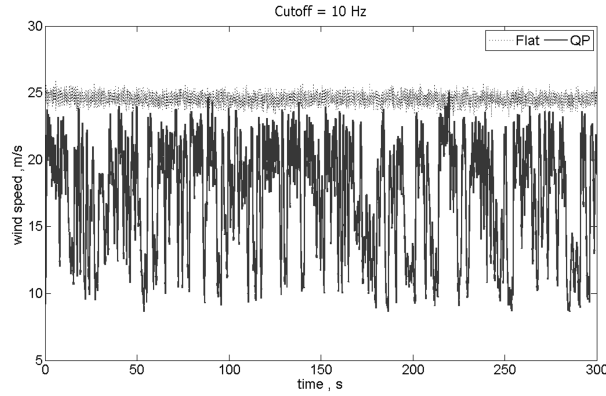
Fig. 5 Time history of flat flow (without low-frequency content), and quasi-periodic (QP) flow (with Low-Frequency Content)
